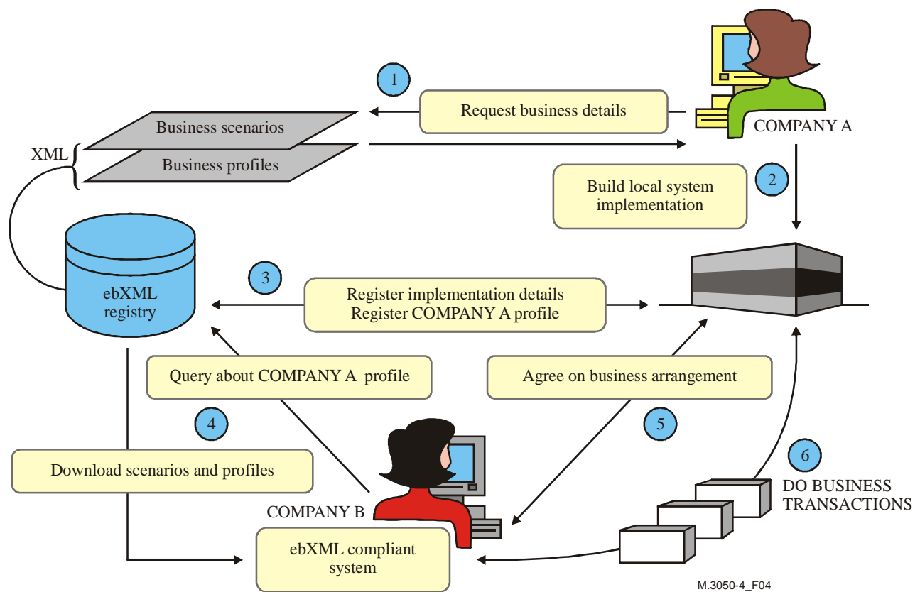
Figure 4/M.3050.4 – ebXML concept
