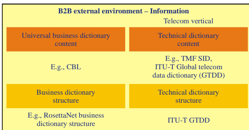
Figure 7/M.3050.4 – eTOM public B2B BOM – Information
