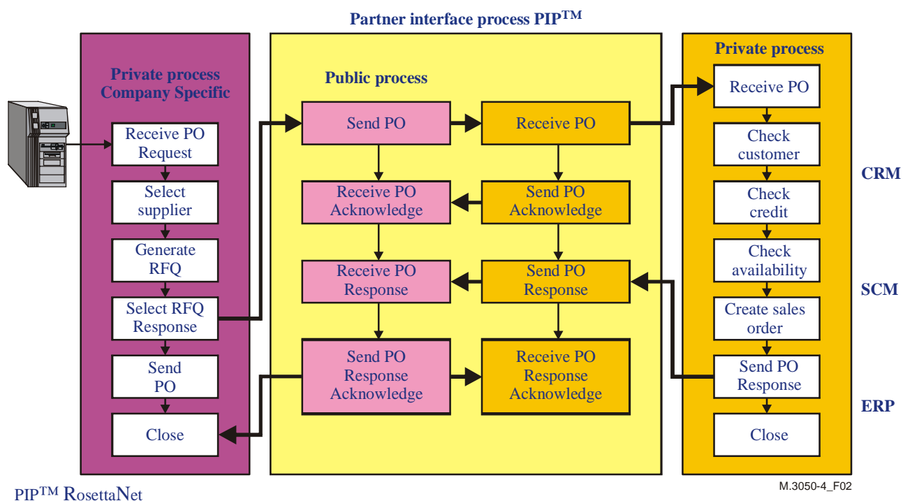
Figure 2/M.3050.4 – Concept of a public process
