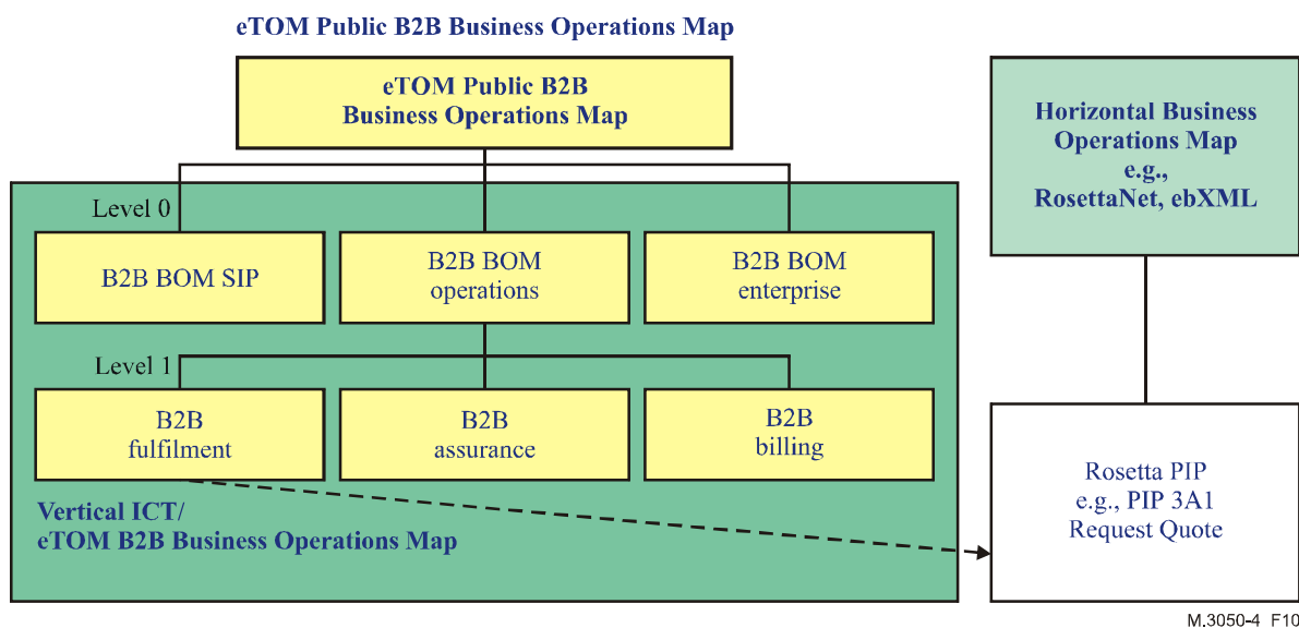
Figure 10/M.3050.4 – eTOM Public B2B Business Operations Map Level 0 and 1
