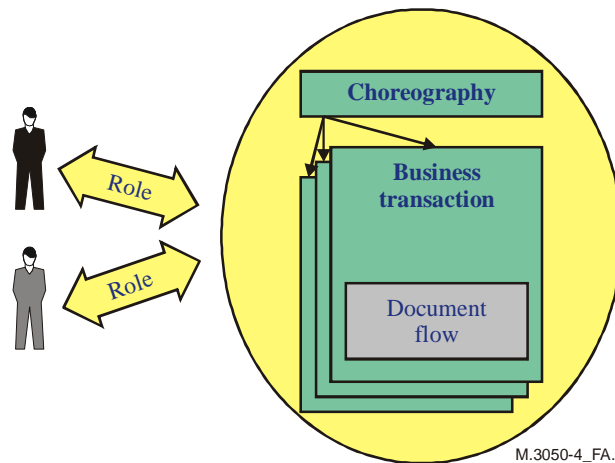
Figure A.1/M.3050.4 – BPSS model business transactions
