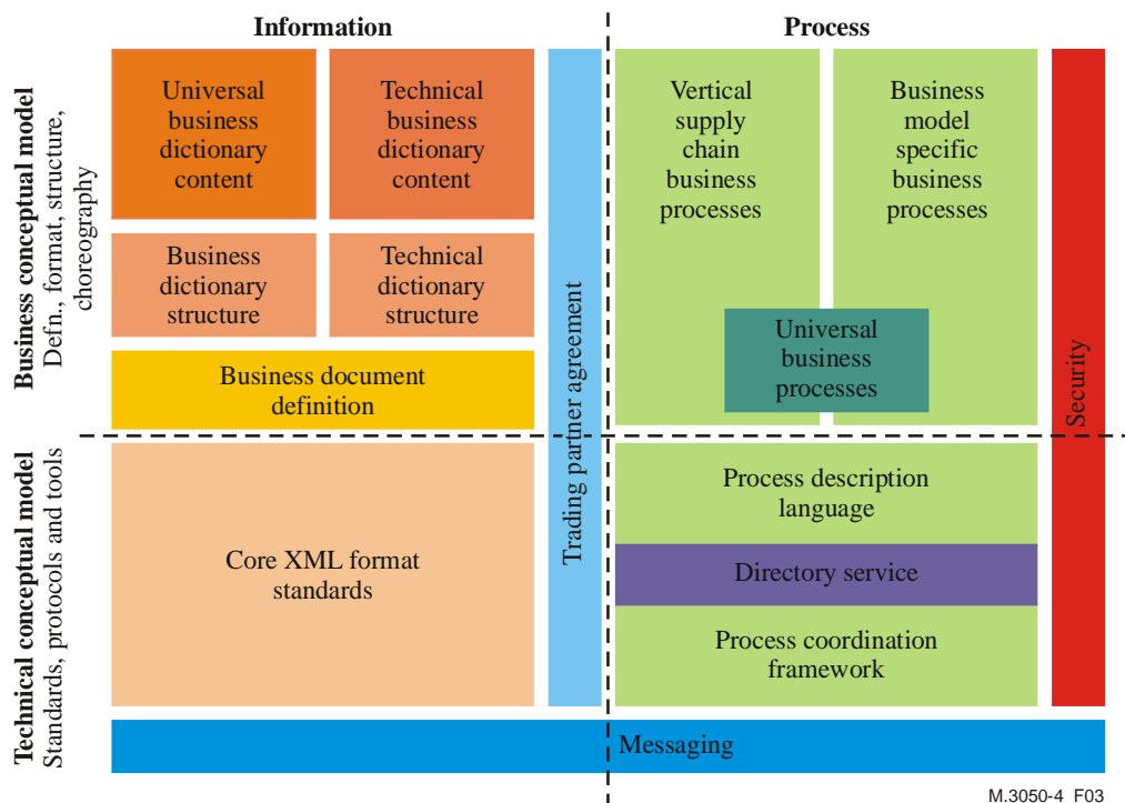
Figure 3/M.3050.4 – RosettaNet conceptual model
