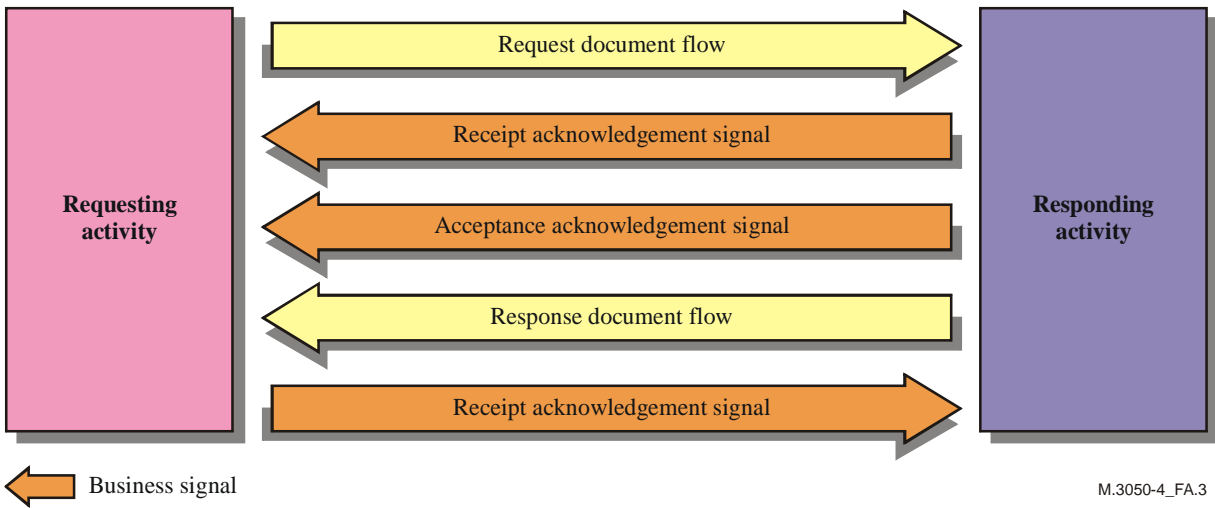
Figure A.3/M.3050.4 – Business documents and business signals
