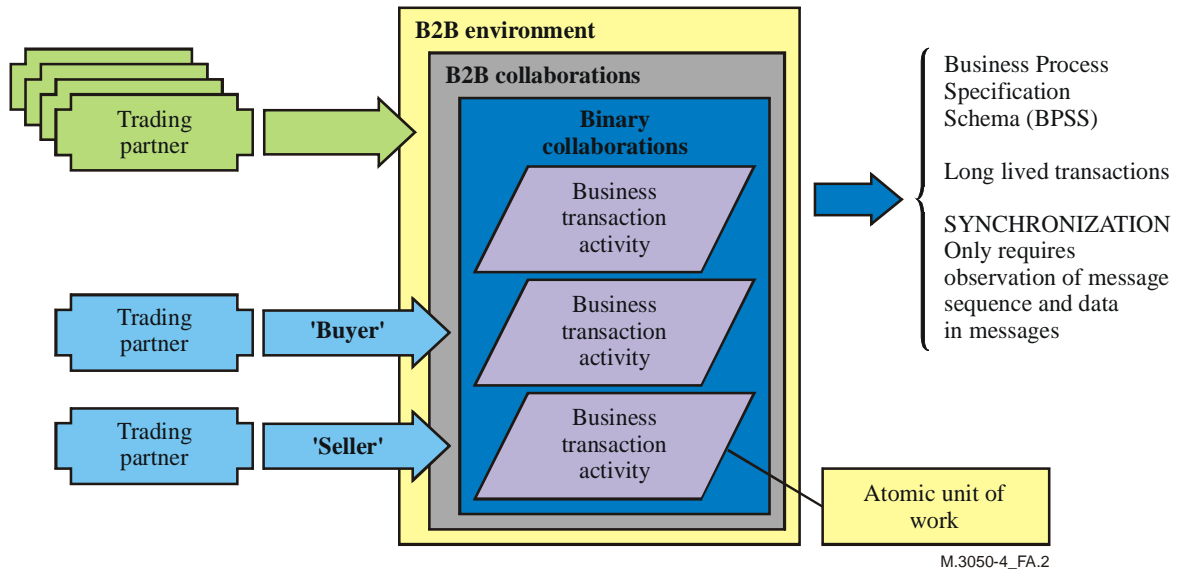
Figure A.2/M.3050.4 – From multiparty collaborations to business transactions
